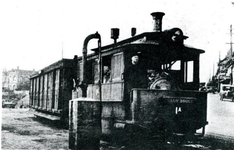
MOTOR 1A AT KOGARAH STATION
